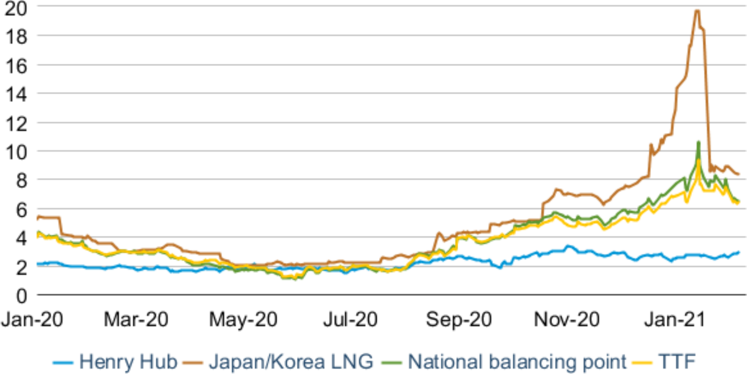
Figure 8. International natural gas prices dollars per million British thermal units
